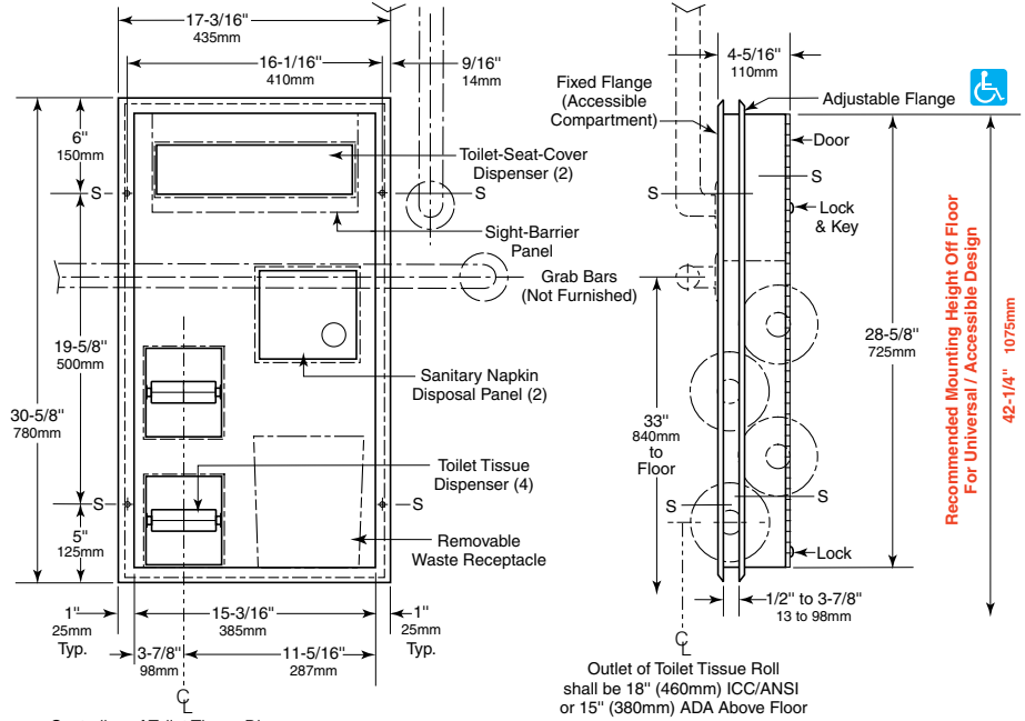
Centerline of Toilet Tissue Dispenser shall be 7" to 9" (180 to 230mm) in Front of Toilet
